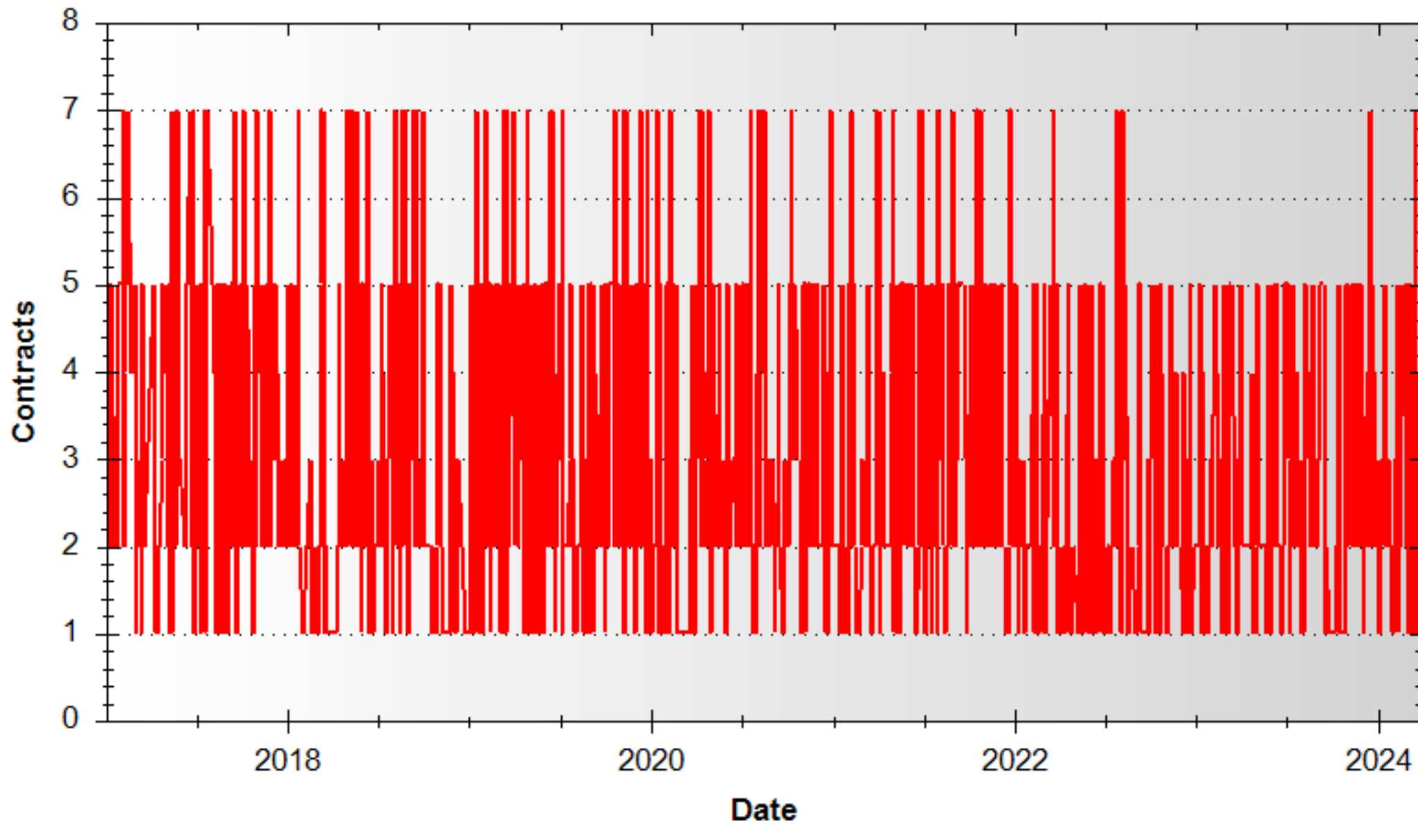
Contracts Traded
