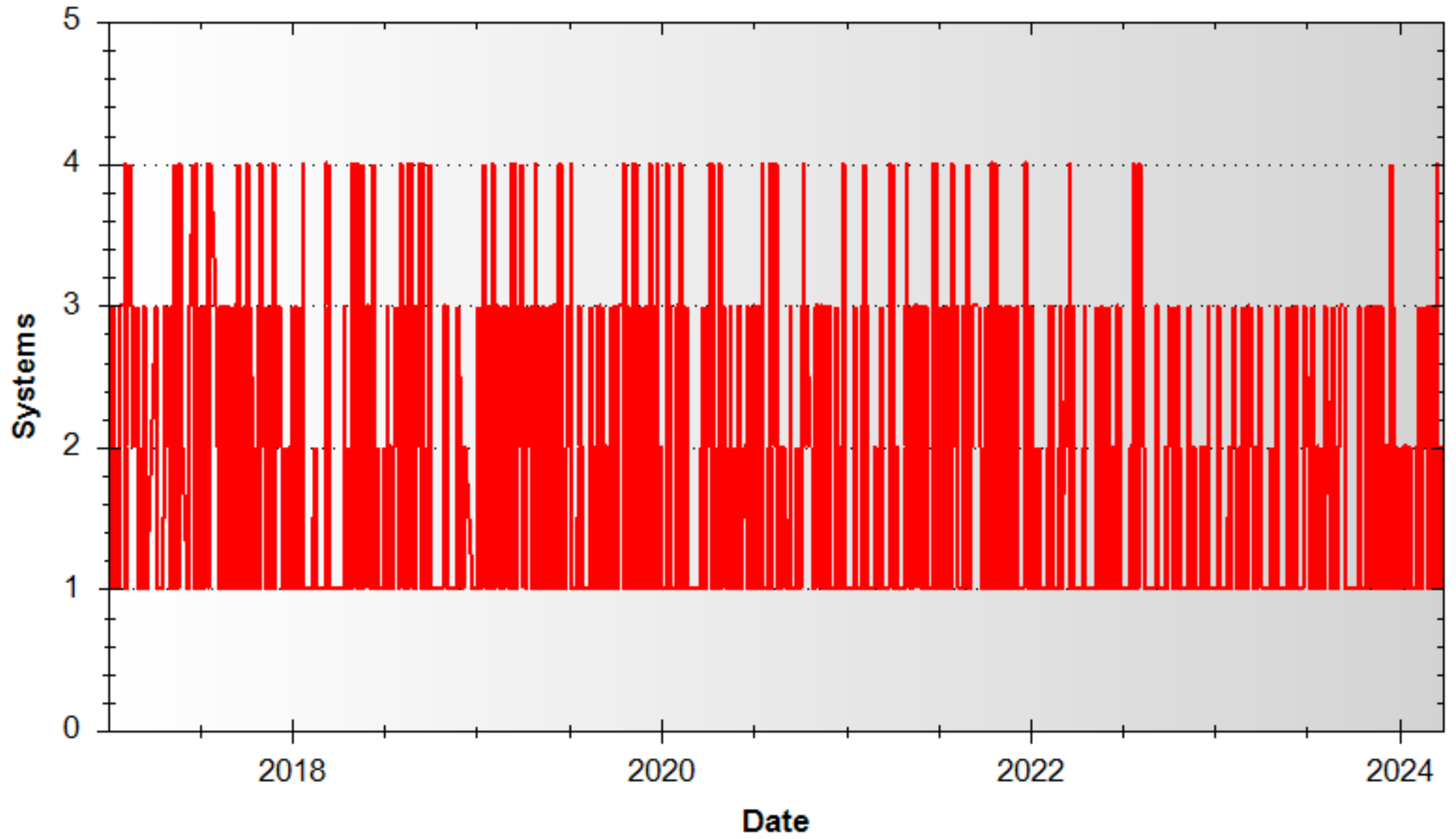
Systems Traded
